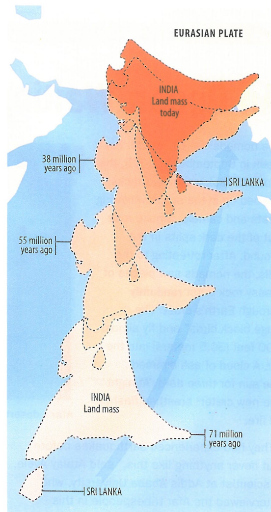
Movement of the India land mass over the past 71 million years
