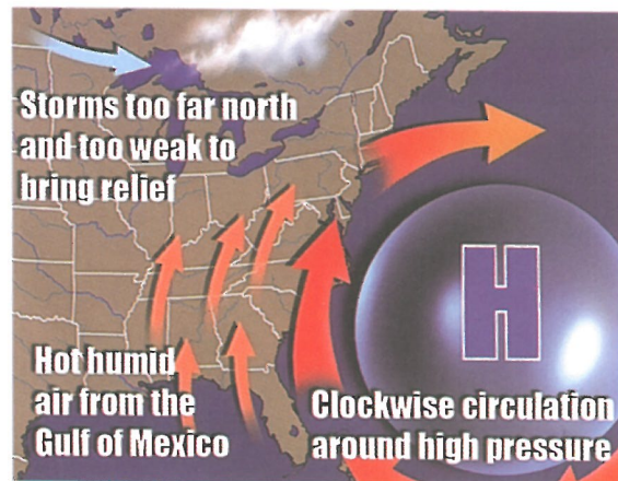
Bermuda High off the U.S. coast
