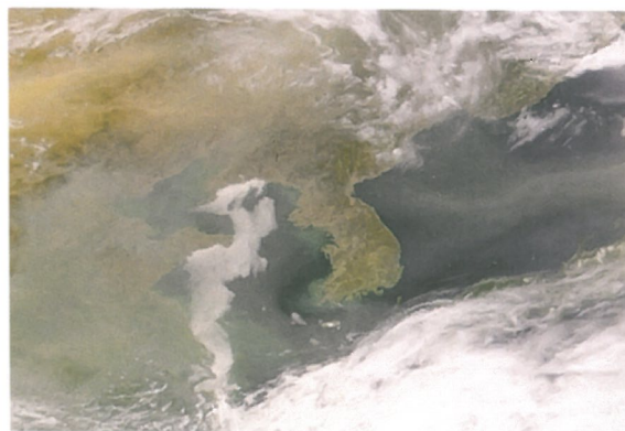
Satellite photos can provide evidence of weather events.
